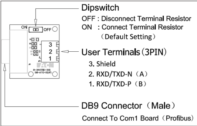
Figure 18. Com1 PROFIBUS DB9 adapter.
