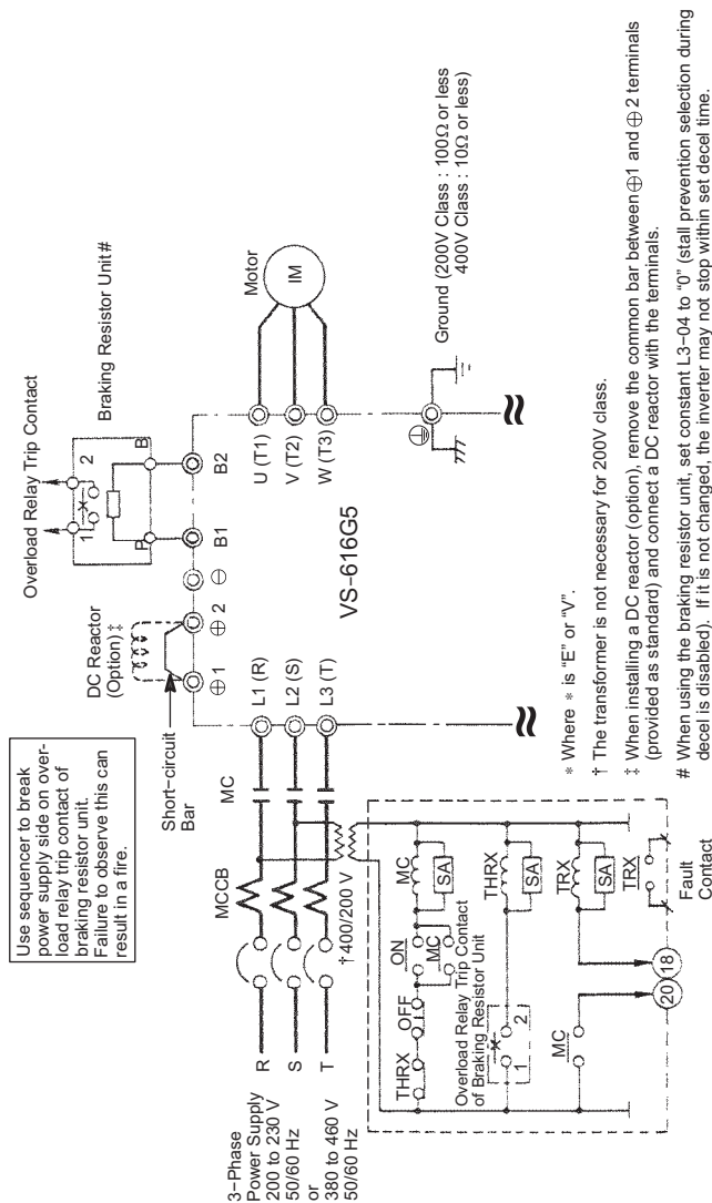
Fig. 14 For Models CIMR-G5*20P4 to -G5*27P5 (200 V Class 0.55 to 7.5 kW), Models CIMR-G5*40P4 to -G5*40I5 (400 V Class 0.4 to 15 kW)
