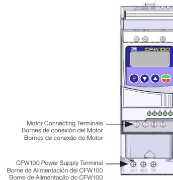
Figure A4: Indication of the connecting terminals of the CFW100
