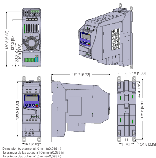
Figure A6: Dimensions of the CFW100 with the RFI filter kit
