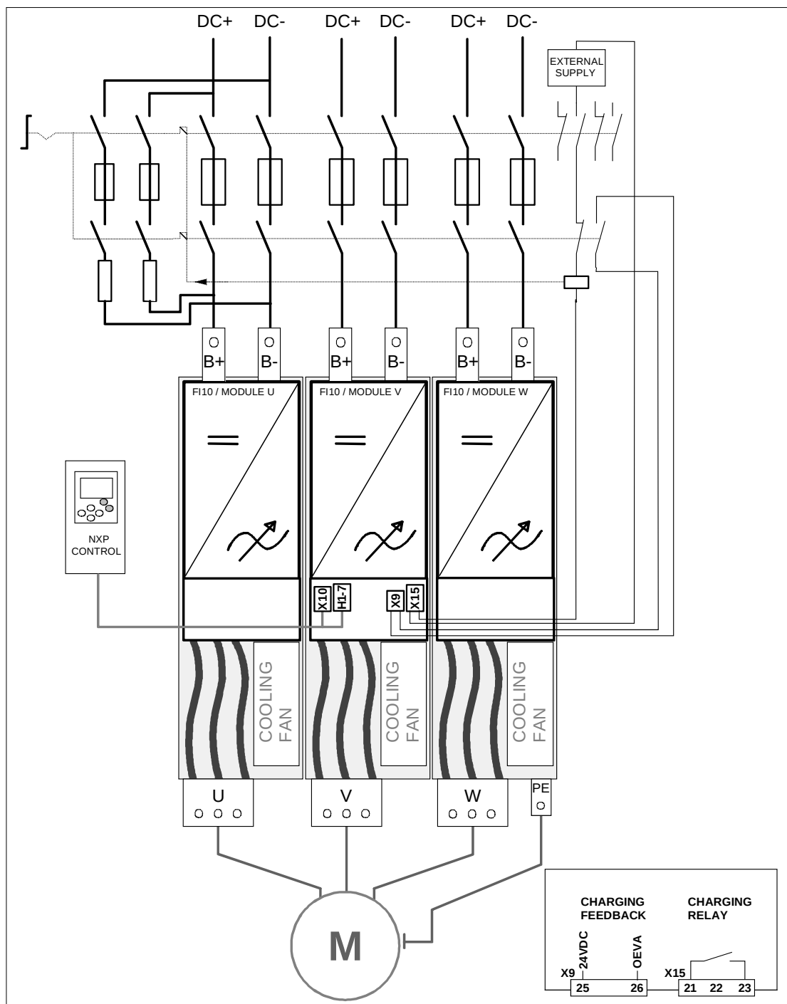
Figure 6-6. FI13 basic wiring diagram with charging
