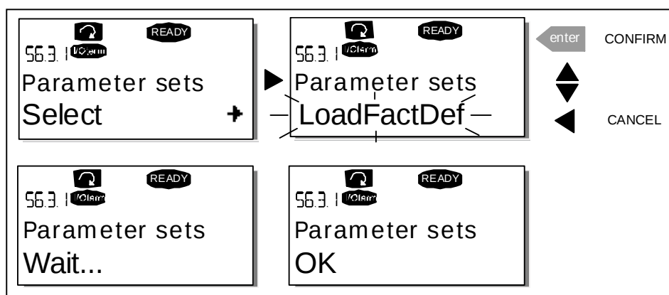
Figure 7-7. Storing and loading of parameter sets
