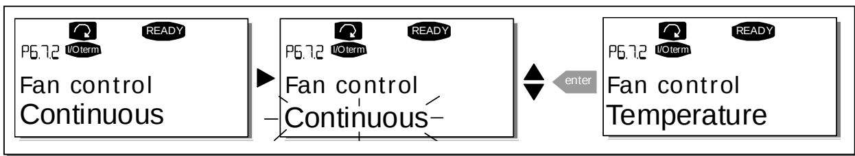
Figure 7-18. Fan control function
