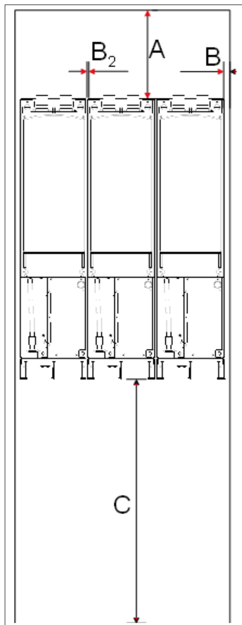
Figure 5-7. Installation space.
