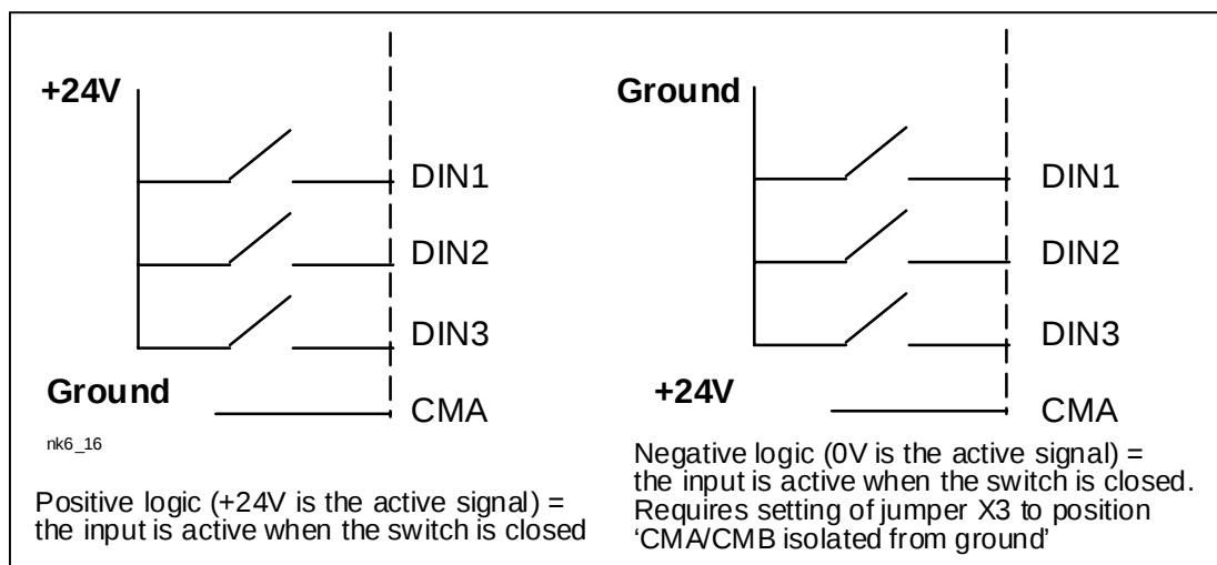
Figure 6-19. Positive/Negative logic
