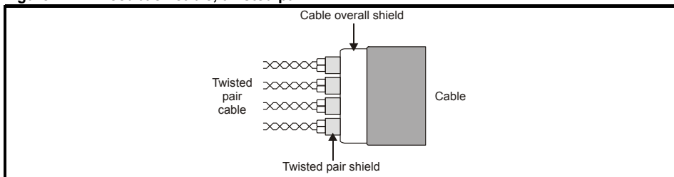
Figure 4-18 Feedback cable connections
