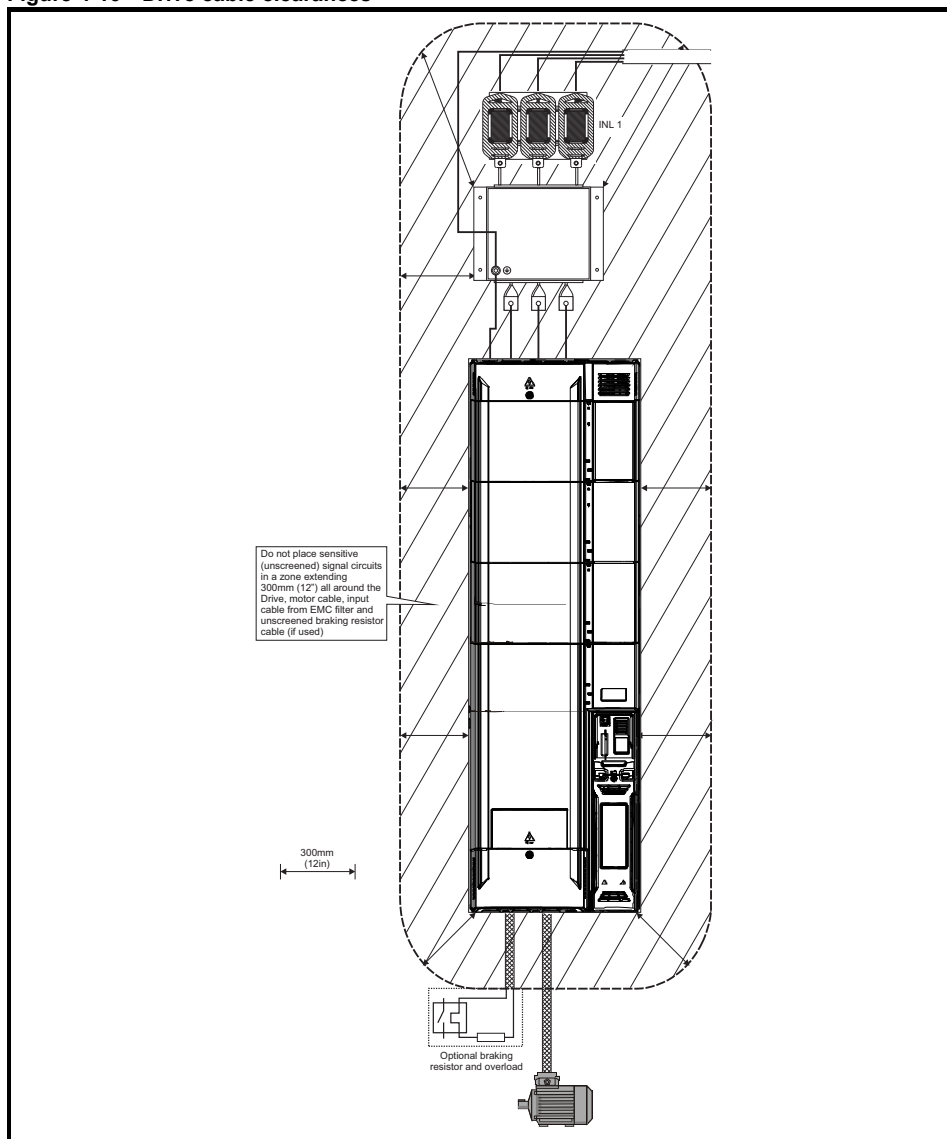
Figure 4-16 Drive cable clearances
