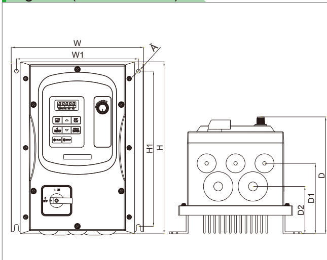
Figure I (IP66 Frame 1)
