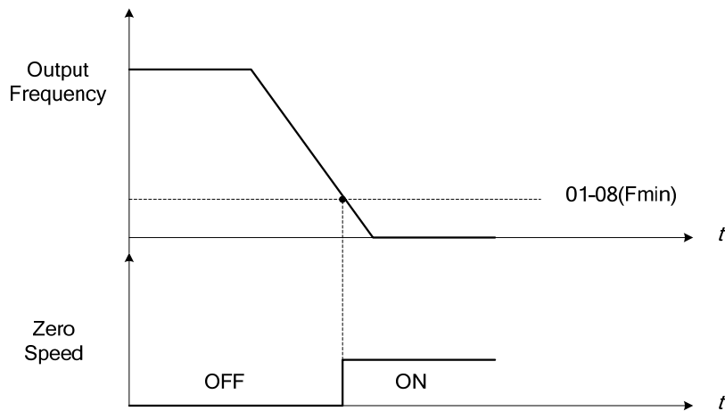
Figure 4.4.26 Zero-speed operation
