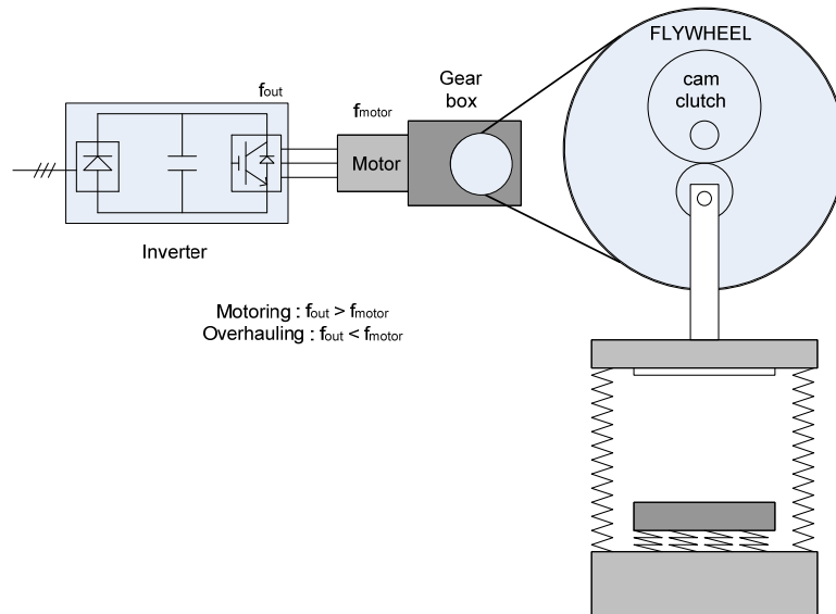
Figure 4.4.91 Stamping Operation
