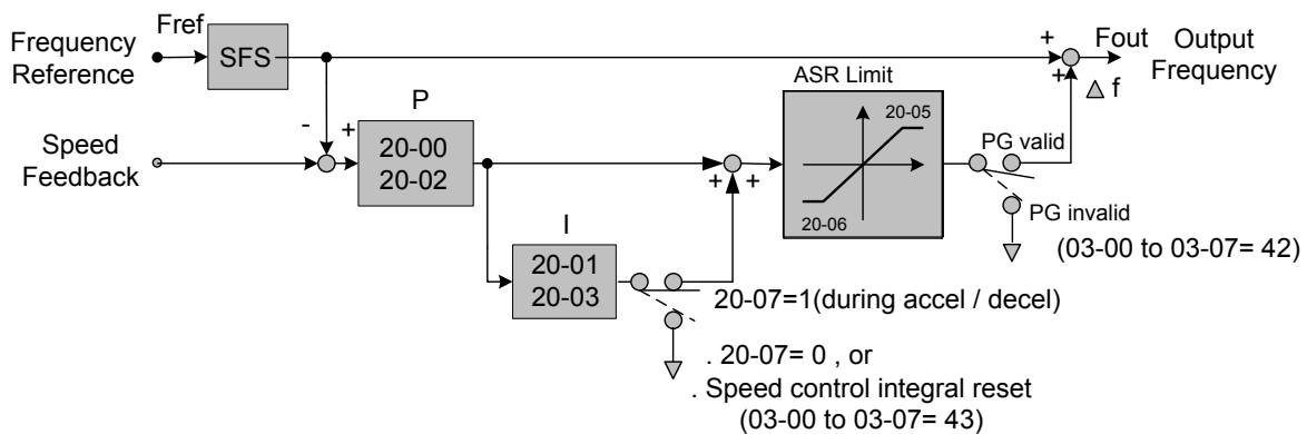
Figure 4.4.108 ASR block diagram (V/F + PG)
