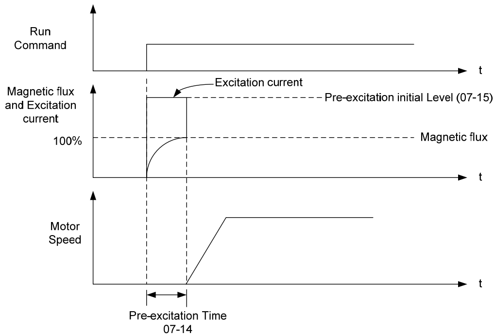
Figure 4.4.63 Pre-excitation operation
