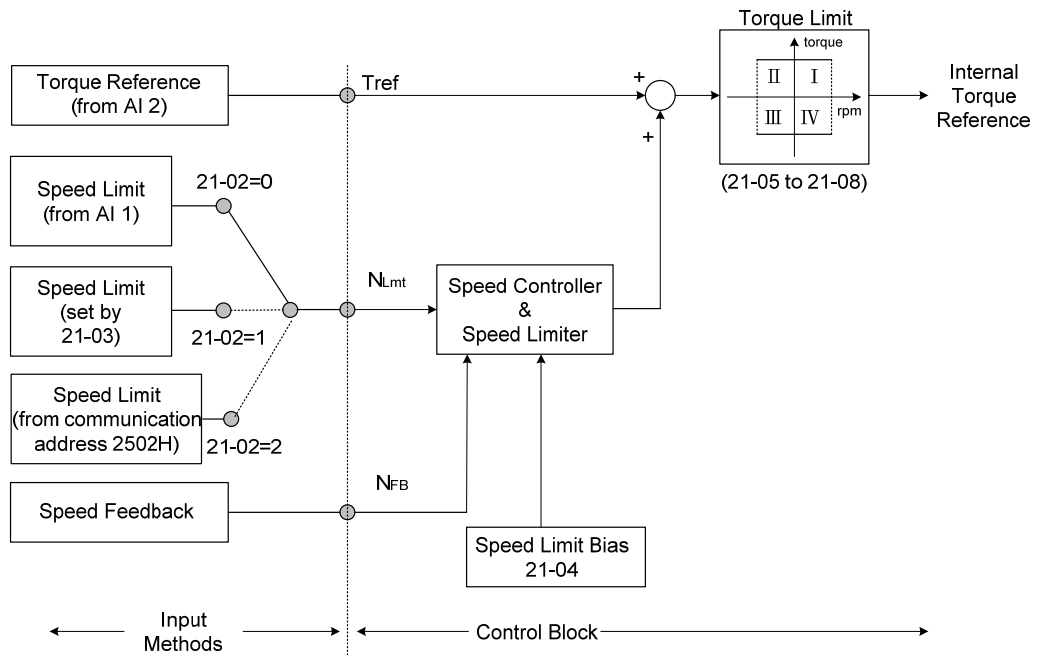
Figure 4.4.122 Block figure of the torque control
