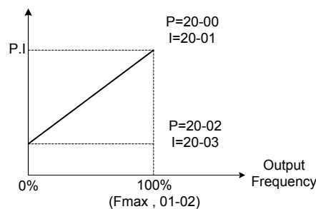
Figure 4.4.111 ASR gain setting (V/F+PG)
