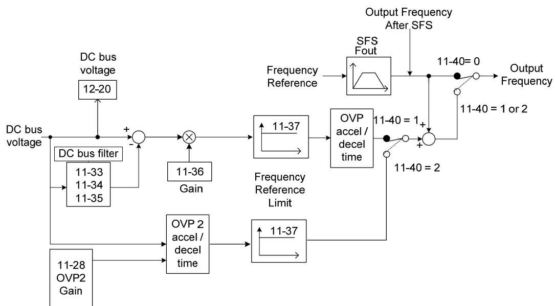
Figure 4.4.92 OVP operation
