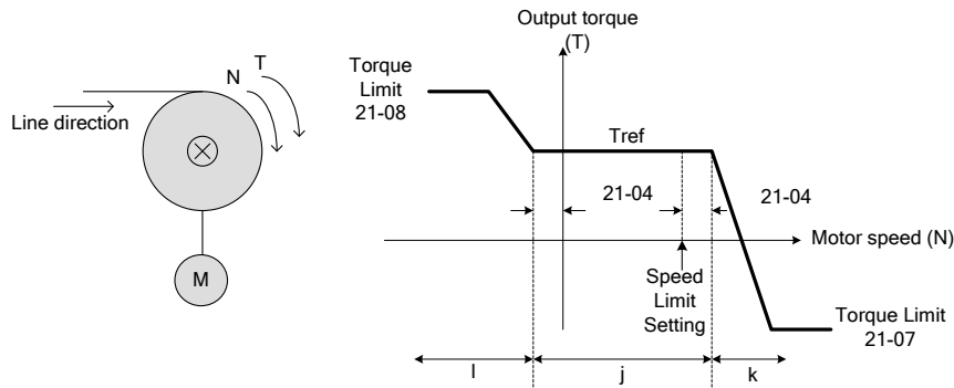
Figure 4.4.125 Winding operation
