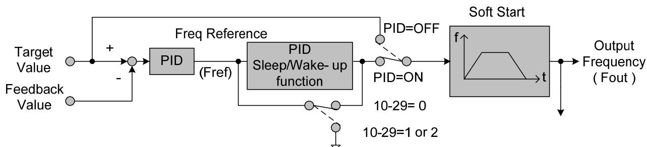
Figure 4.4.84: (a) PID control block diagram
