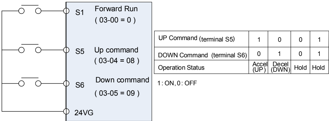
Figure 4.4.19 UP/DOWN wiring and operation example
