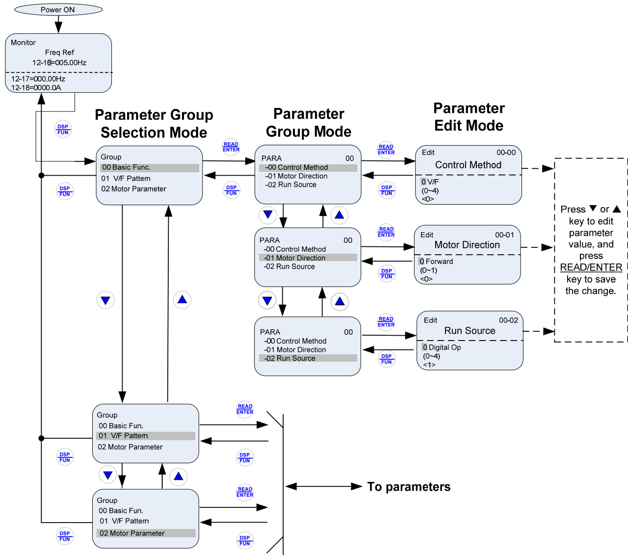
Fig 4.2.2.3 Programming Mode
