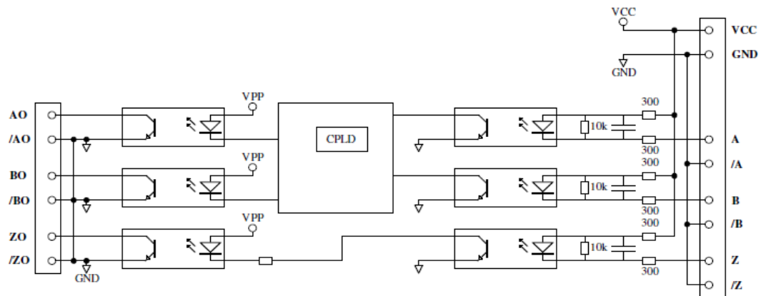
JN5-PG-O block diagram:
