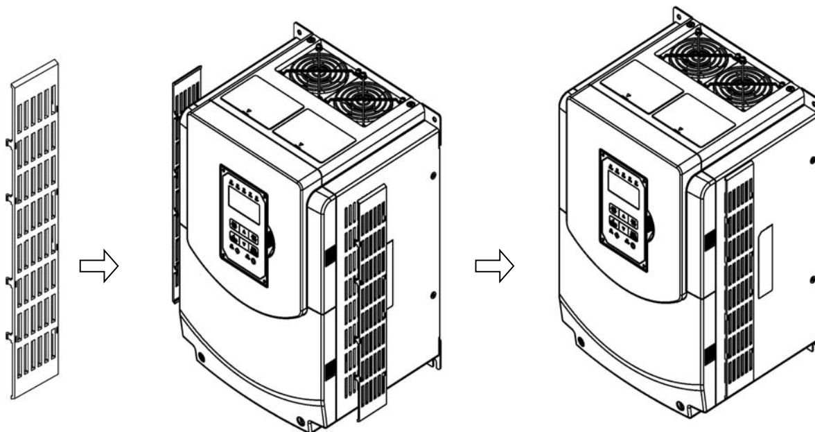
Protective Cover
