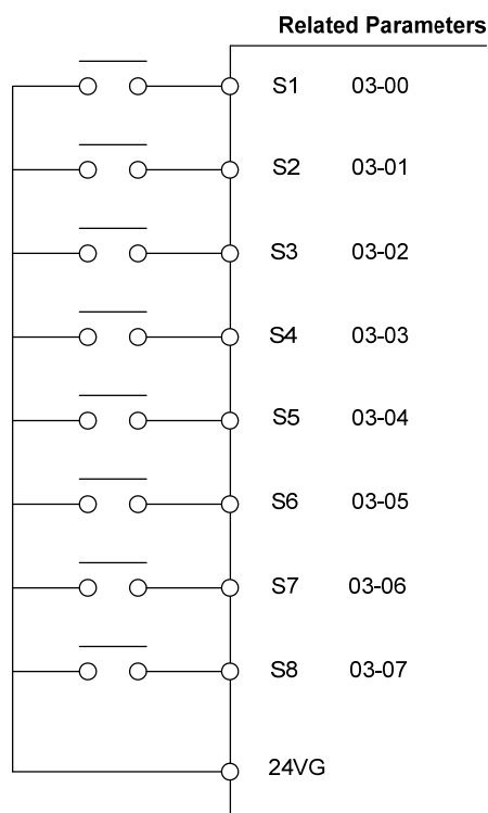
Figure 4.4.16 Multi-function digital input and related parameters
