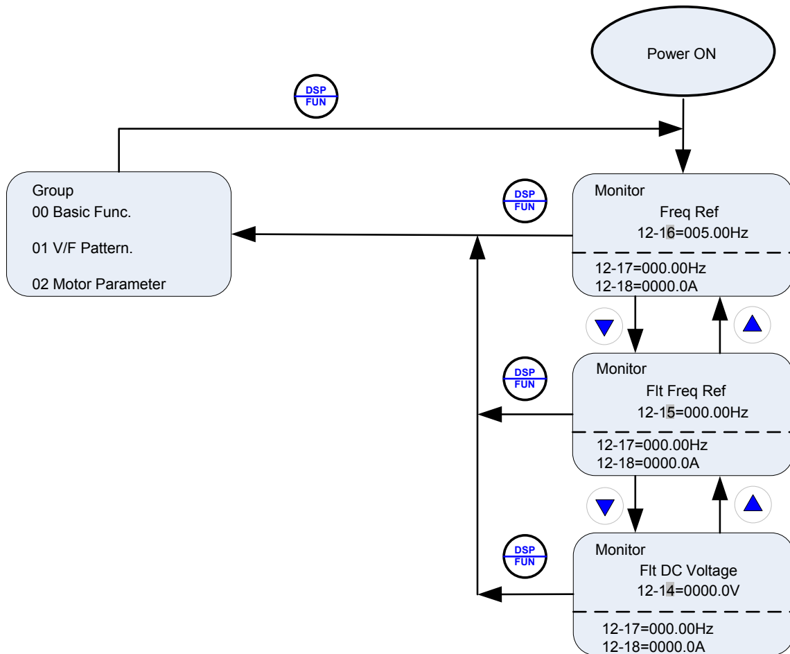
Fig 4.2.2.2 Monitor Mode
