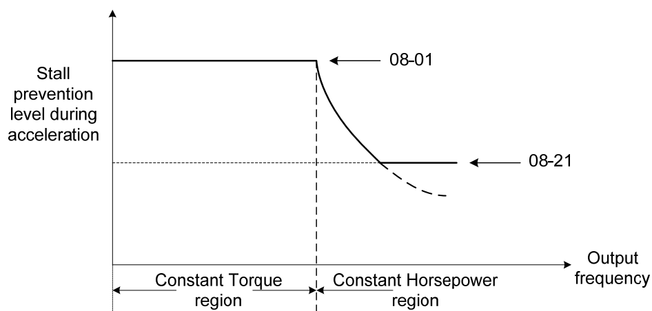
Figure 4.4.69 Stall prevention level and limit in acceleration
