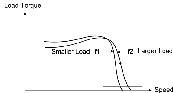
Figure 4.4.100 Slip compensation output frequency
