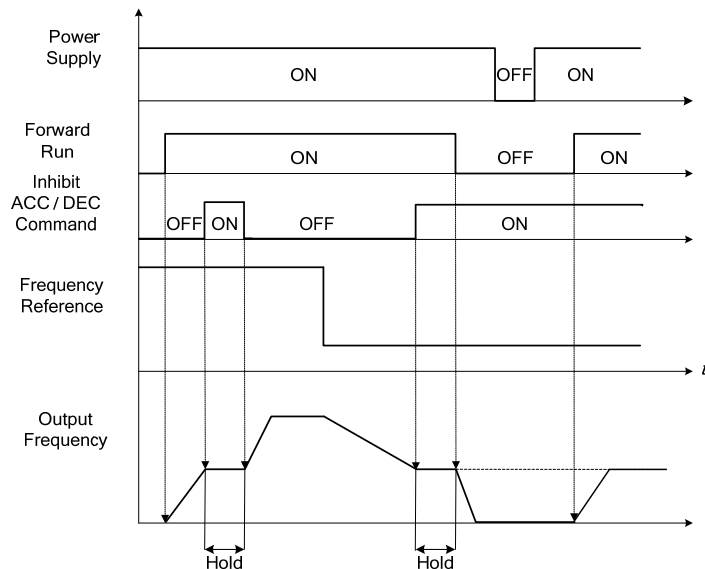
Figure 4.4.21 Acceleration/ deceleration inhibition command operation
