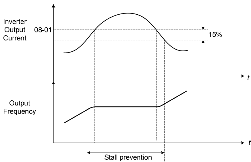
Figure 4.4.68 Stall prevention during acceleration
