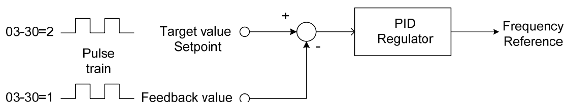
Figure 4.4.28 PID control
