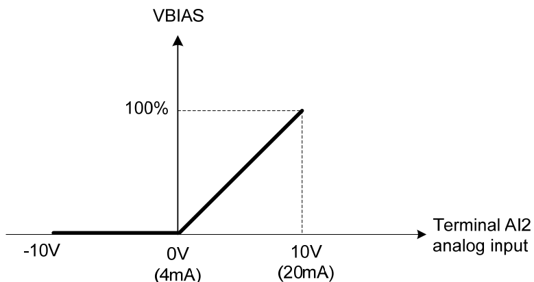
Figure 4.4.42 Bias adjustment
