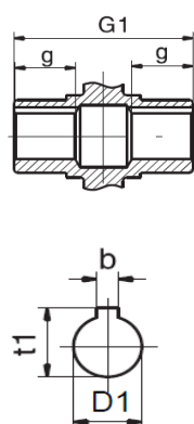
Output Hub
