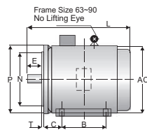
Frame Size 63-90 No Lifting Eye
