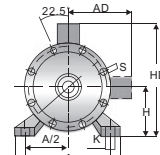
Frame Size 225-355
