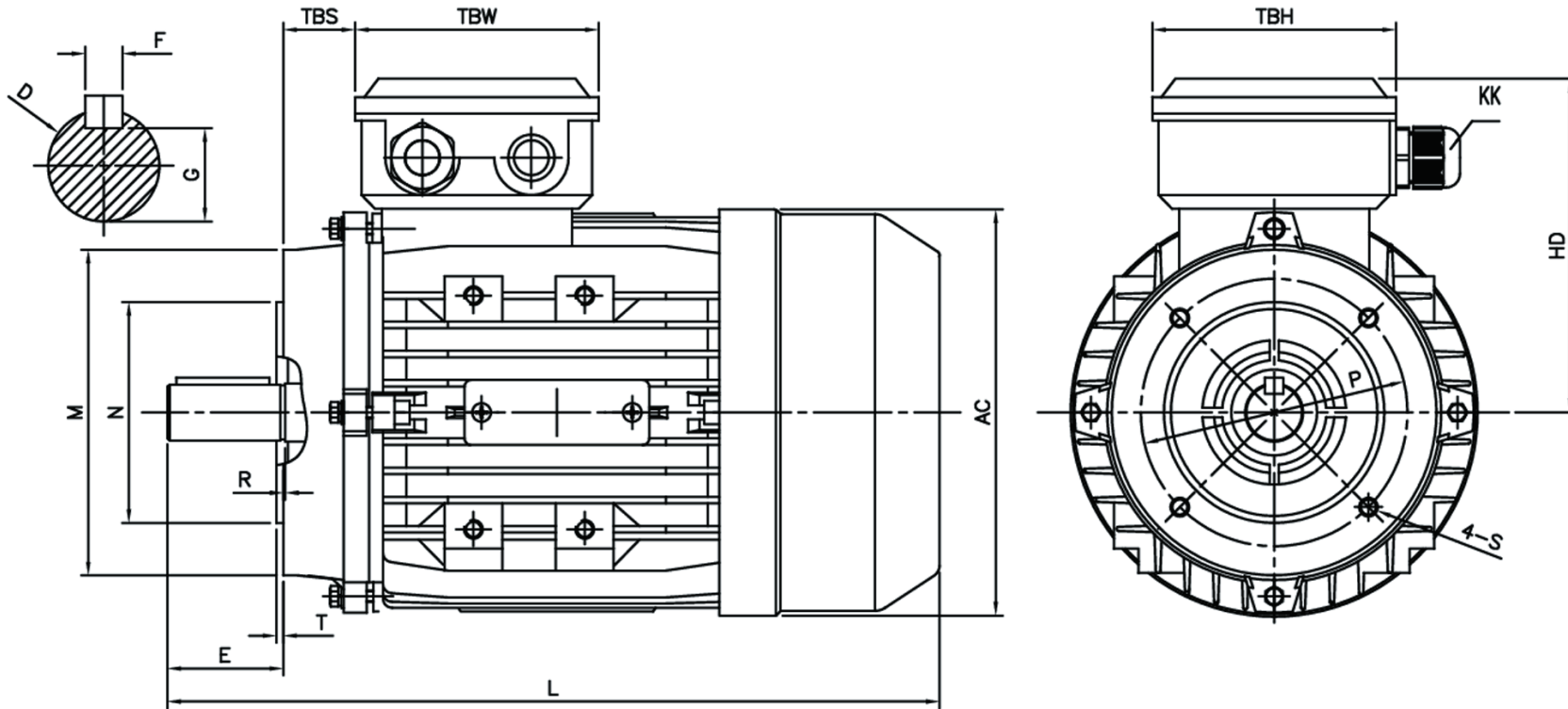
MS56-132 B14 & B14B Overall & Installation Dimension
