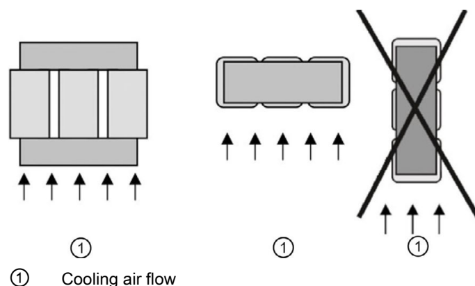
Figure 3-2 Mounting position
