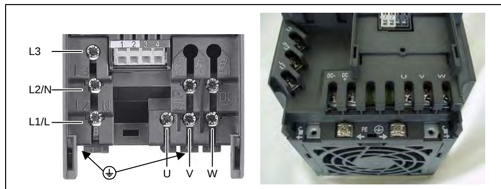
Fig. 1-2 Power Terminals
