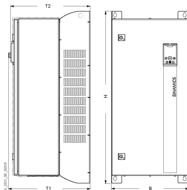
Dimension drawing Power Module PM230, IP55 with integrated line filter A/B
