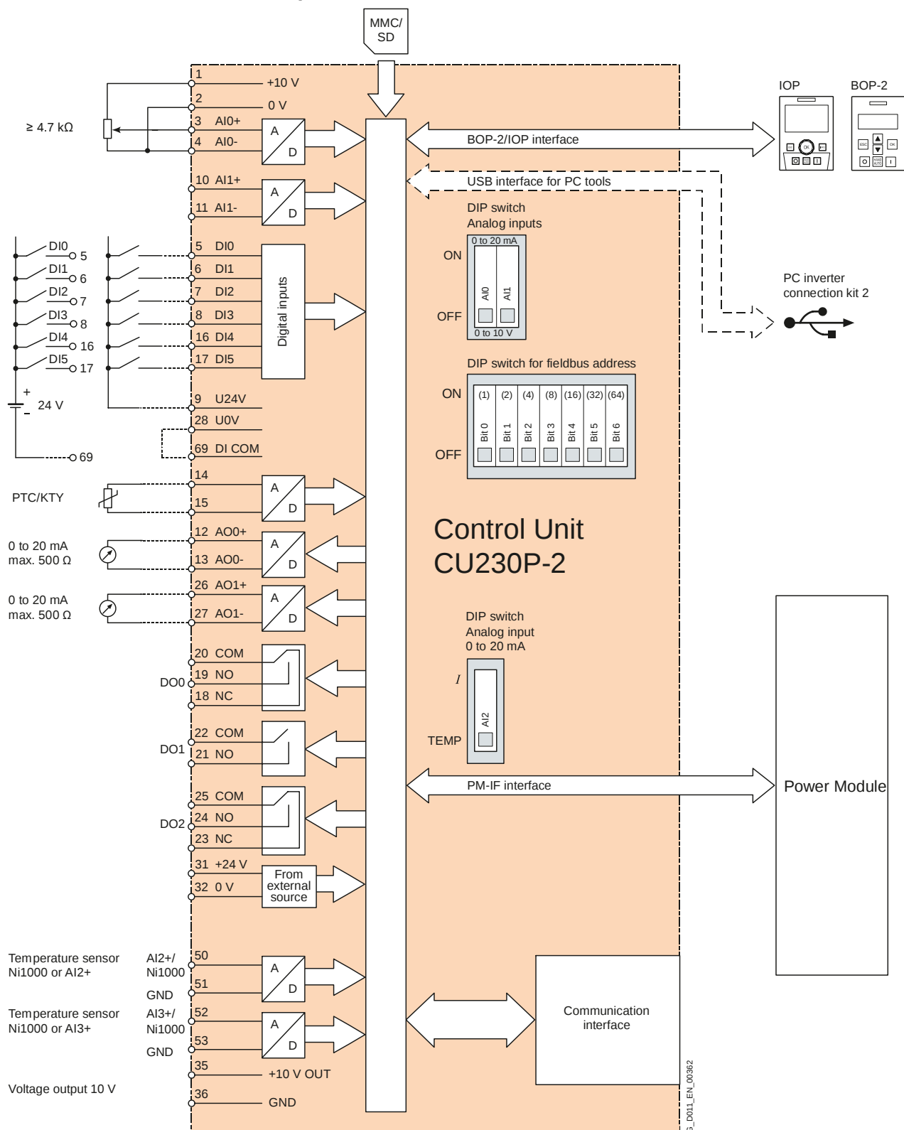
Connection diagram Control Unit CU230P-2 BT
