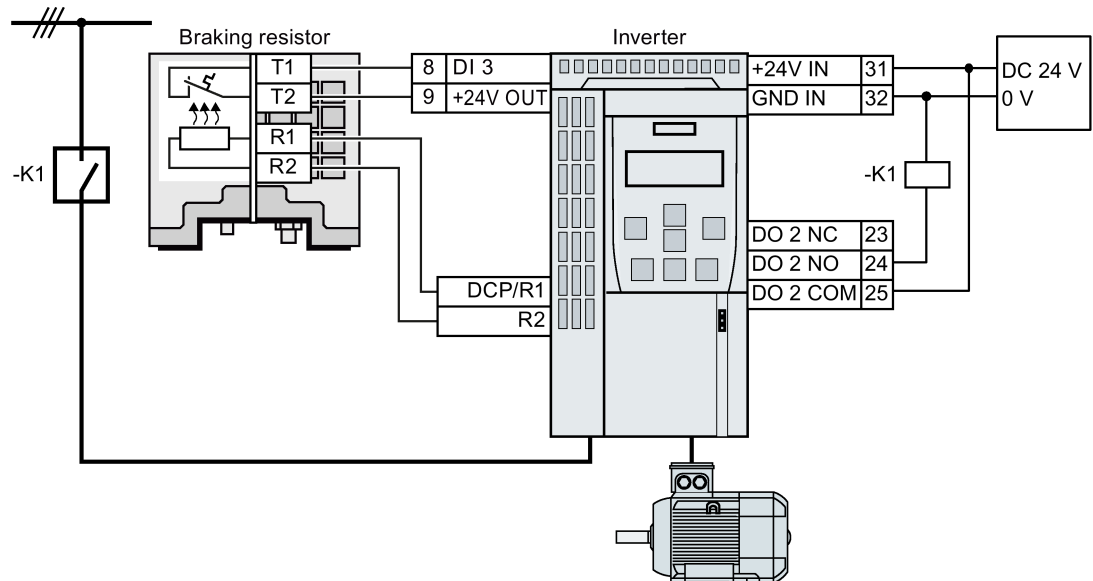
Figure 8-6 Connecting a braking resistor with temperature monitoring via digital input DI 3 and line contactor control (-K1) via digital output DO 2
