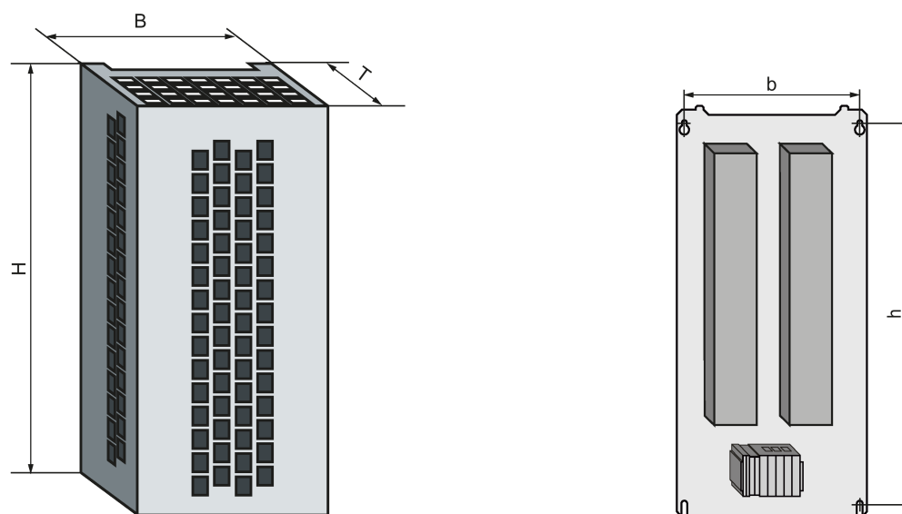
Figure 8-4 Braking resistor
