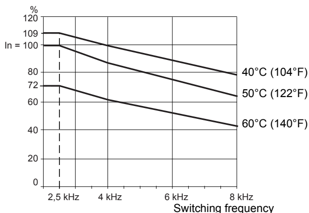
ATV71HC20N4
