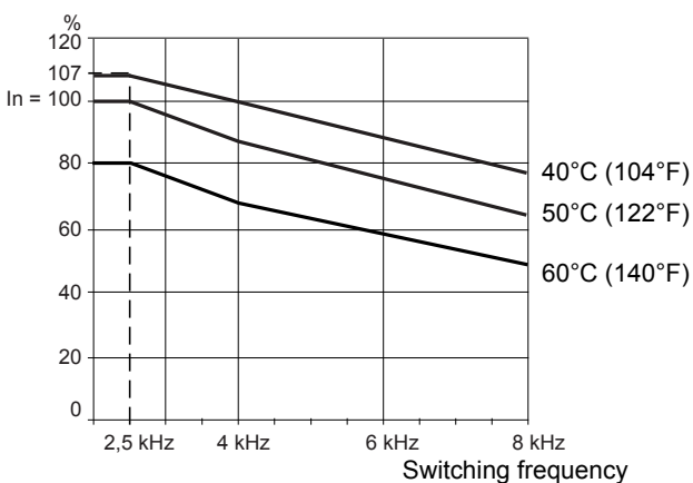
ATV71HC40N4
