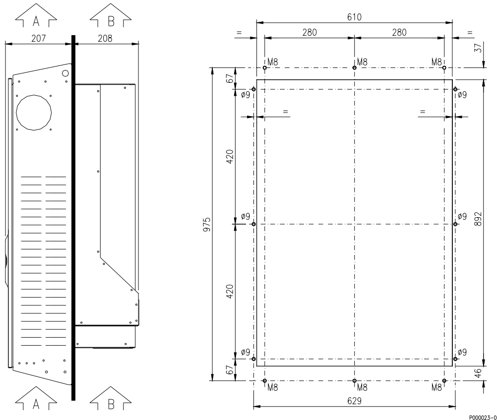
Figure 21: Through-panel assembly and fixing points for SINUS K S50.
