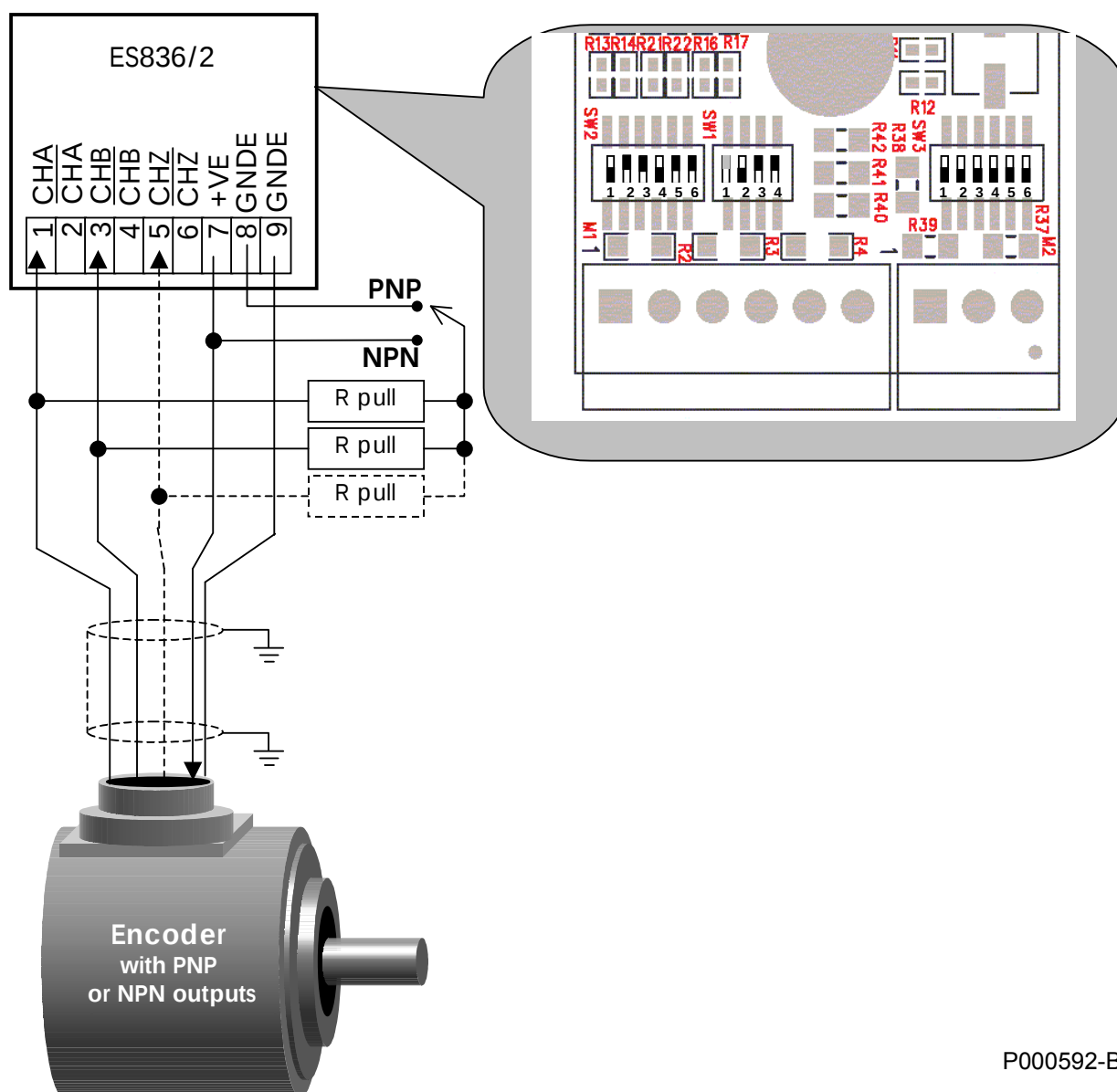
Figure 83: PNP or NPN encoder with single-ended outputs and load resistors with external wiring.
