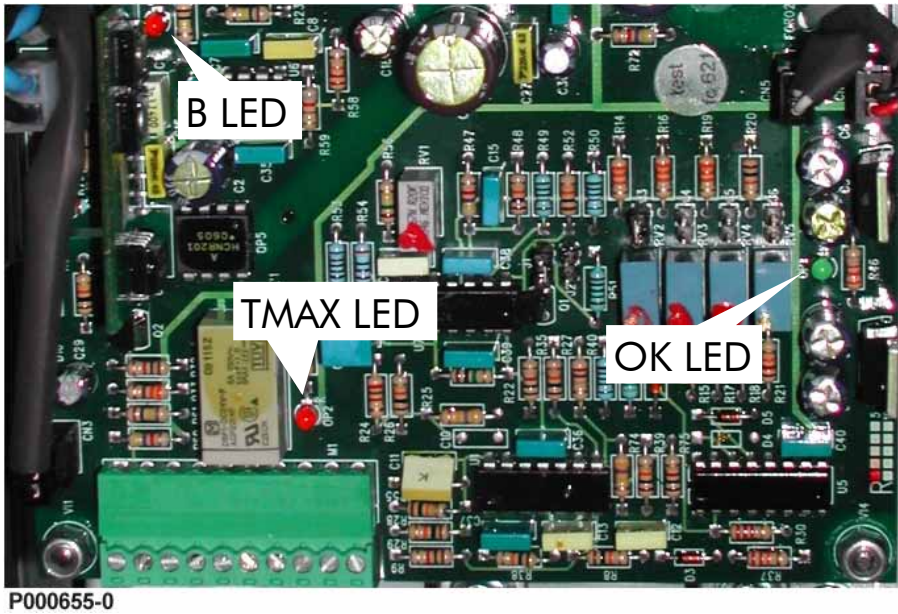
Figure 56: Position of the indicator LEDs.
