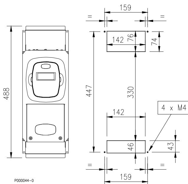
Figure 12: Fixing points of the mounting panel for the through-panel assembly of SINUS K S05.
