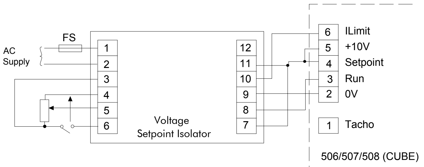
Figure 5 Current Control
