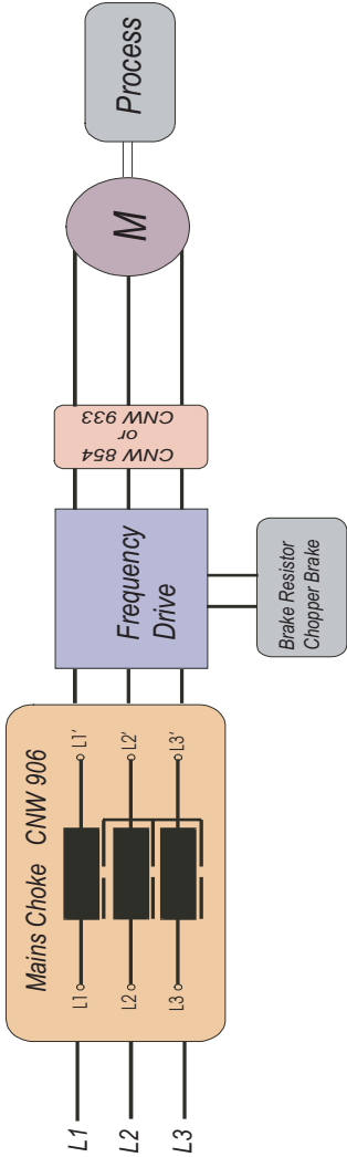
Circuit Diagram
