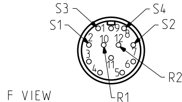
FEEDBACK CONNECTOR
