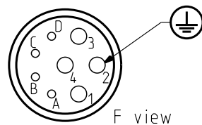
FEEDBACK CONNECTOR
