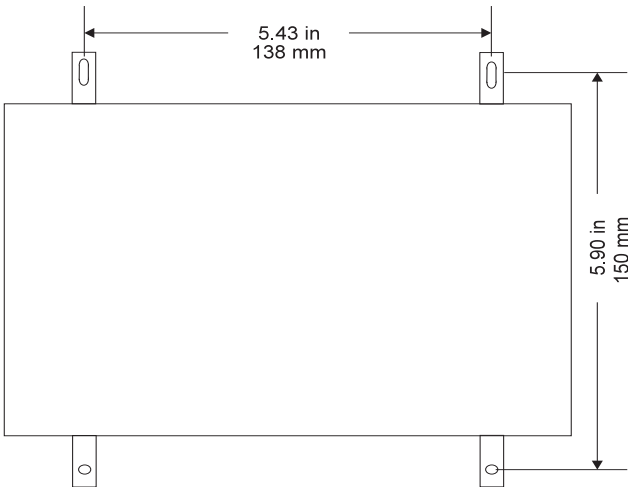
Figure 2 - LinkRack Panel Mounting Detail
