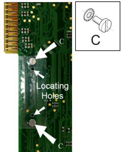
Figure 3 Rear of Control Board
