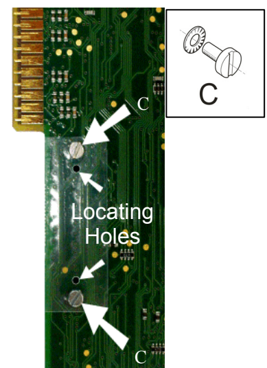
Figure 3 Rear of Control Board
