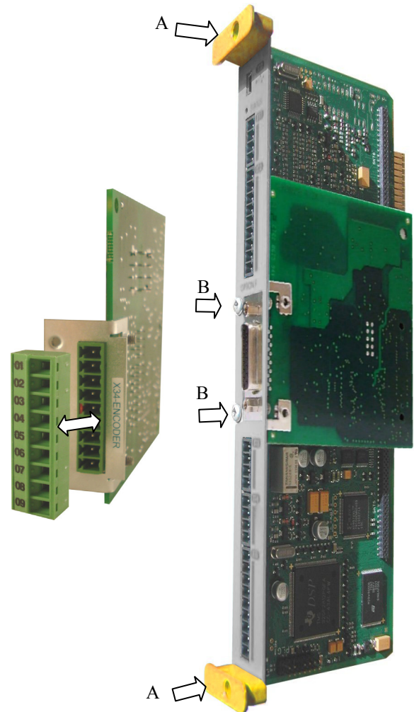
Figure 2 Control board showing Option correctly mounted
