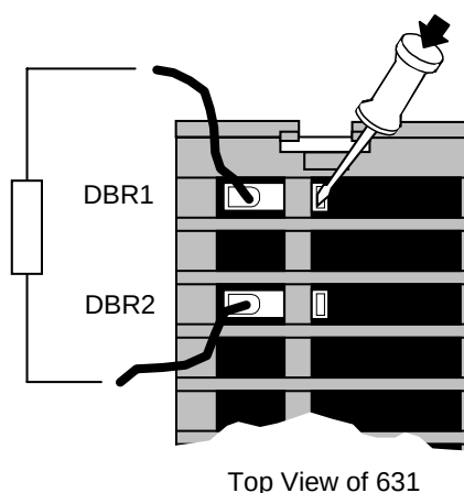
Figure 3-3 External Brake Resistor Terminals
