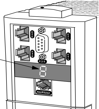
Diagnostic Display
