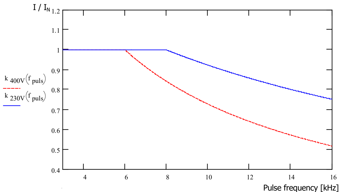
Figure 34: Heat losses due to pulse frequency
