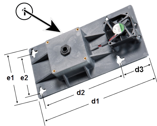
1 Insertion of fan connecting cable
