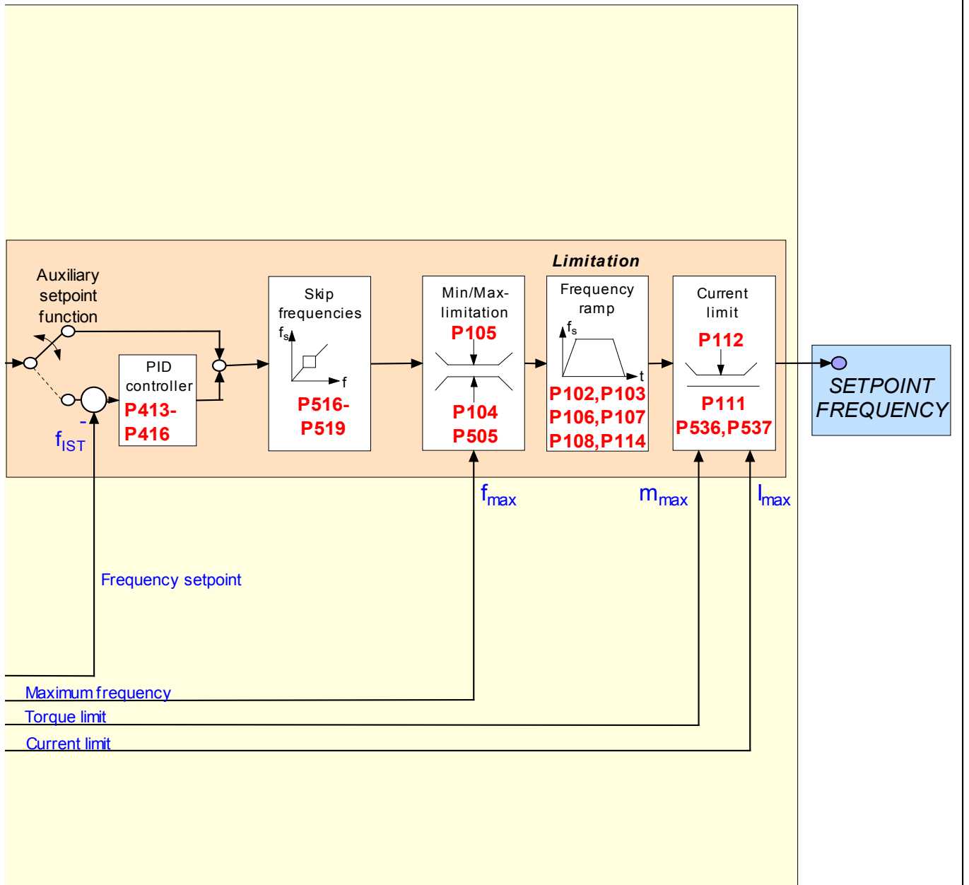
Fig. 14: Setpoint processing
