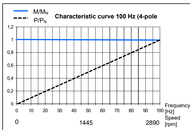
Figure 17: Characteristic curve 100 Hz
