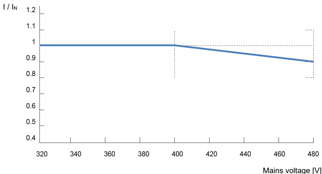
Figure 12: Reduced output current due to low voltage
