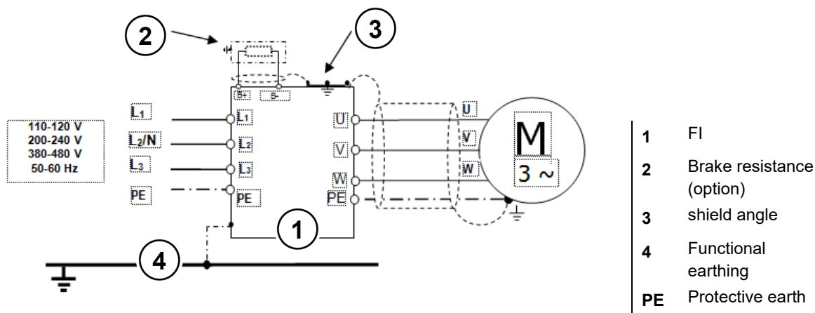
Figure 10: Wiring recommendation
