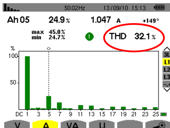
Picture 3: THDI with DC-choke
