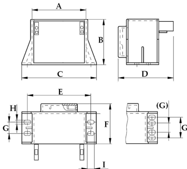
Picture 6: DC-choke, drowned type
