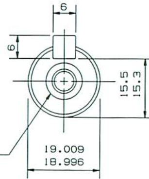
SHAFT END DETAILS
