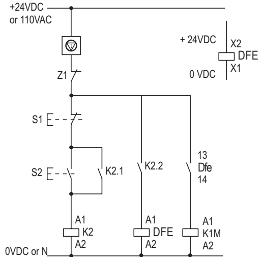
3 wire control 24 VDC/110VAC
