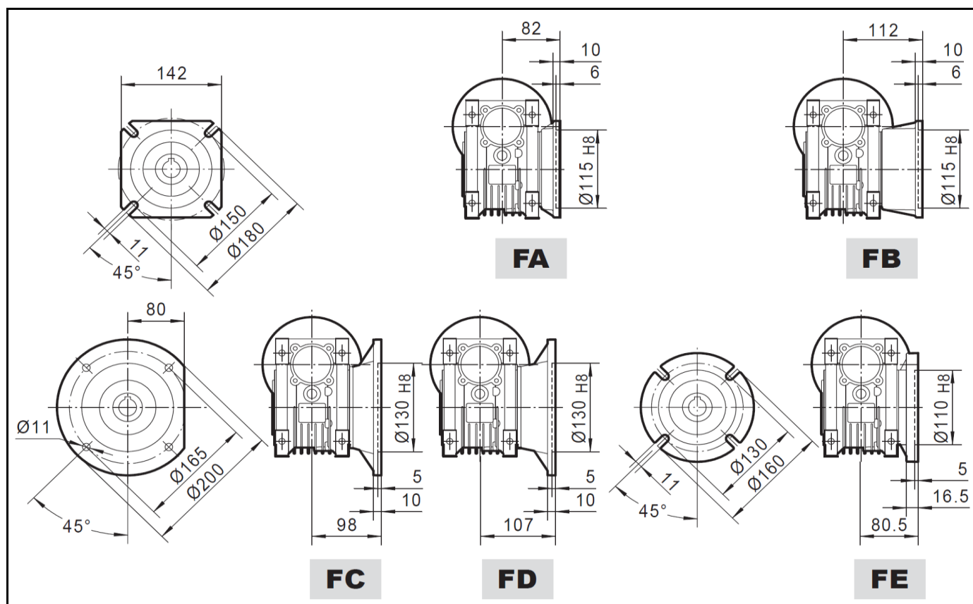
Input Flange & Output Bore Dimensions
