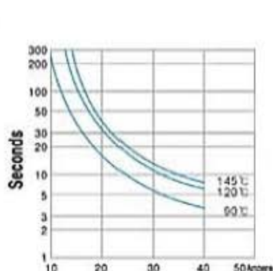
TRIP TIME / CURRENT (AT 25°C)
