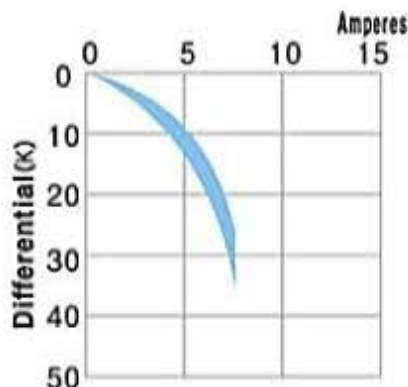
OPEN TEMP. DROP/CURRENT
