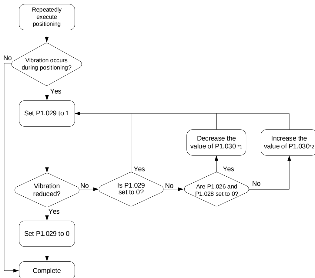
Flowchart of auto low-frequency vibration suppression:
