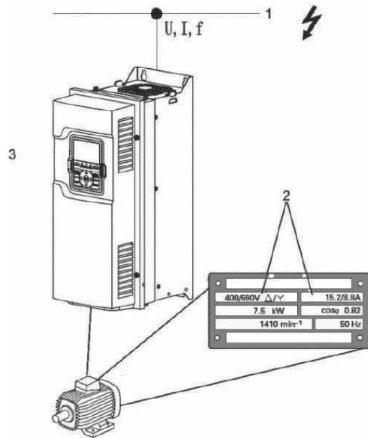
Figure 11. Selection criteria
