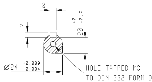
SECTION ON 'X'
