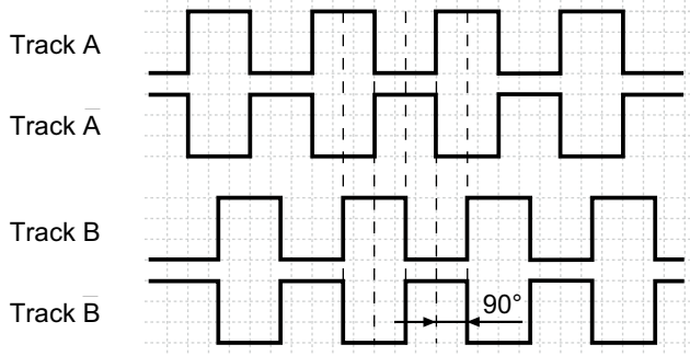
BI-Output signals (Square wave signal-encoder)
