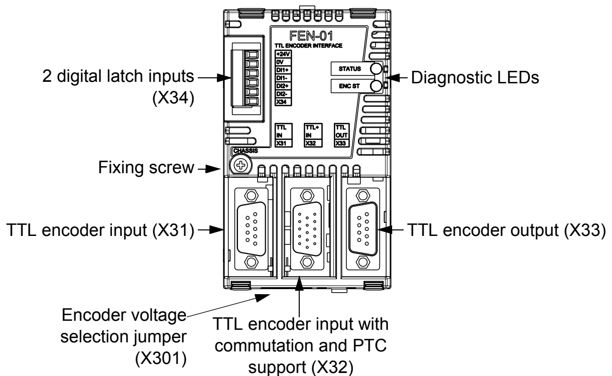
FEN-01 layout
